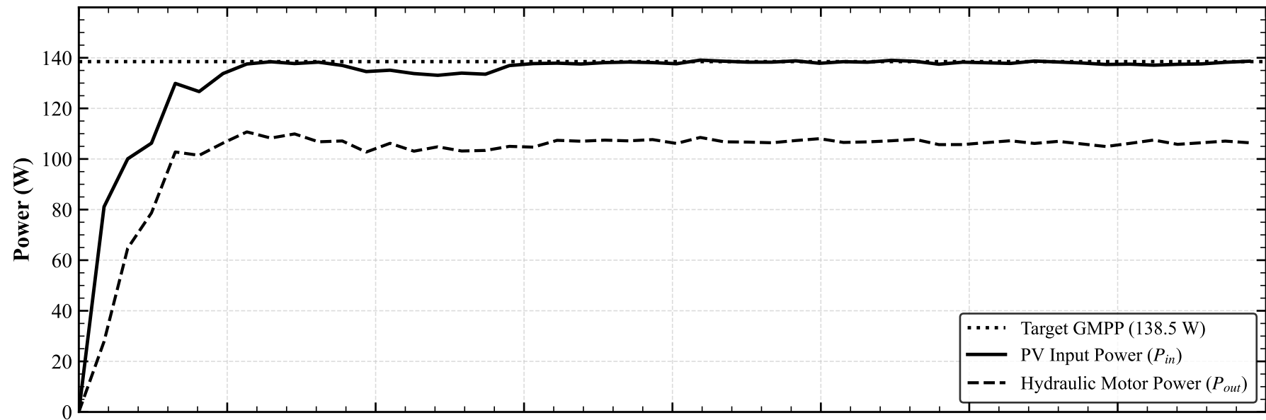
Hydraulic System Response — Level 5 (Non-Shading - STC 1000 W/m 2 )
